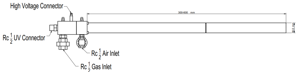
Figure 1: PBA90 Series air burner
